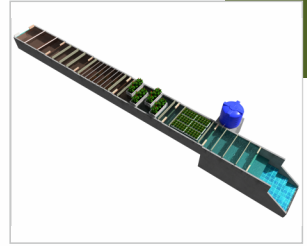
Insitu Nallah Treatment Technology (N-Treat - IIT Bombay IP)
